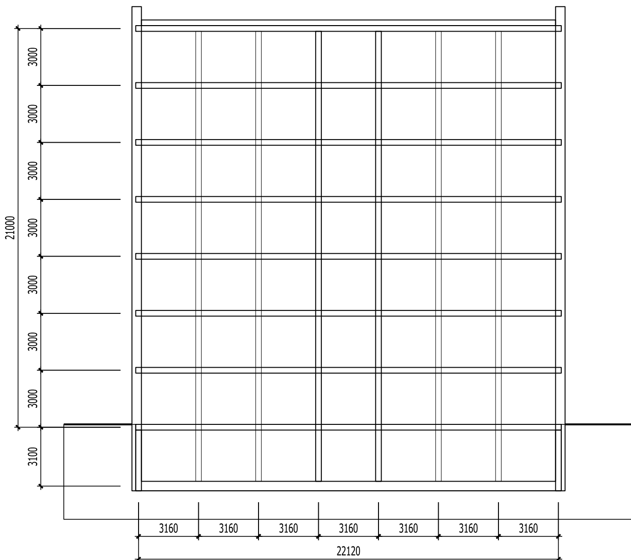
Longitudinal section of the building
