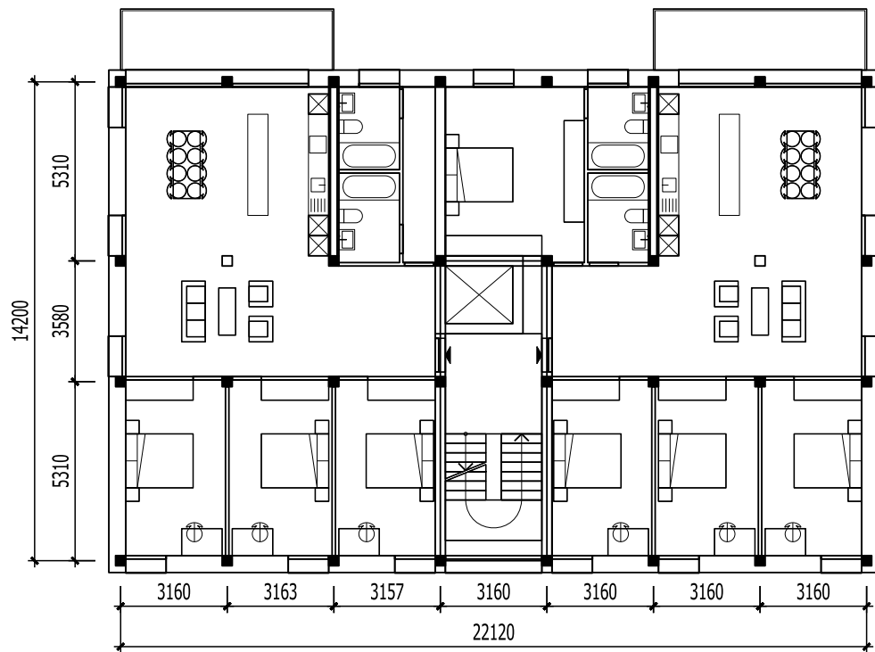
TYPICAL FLOOR
